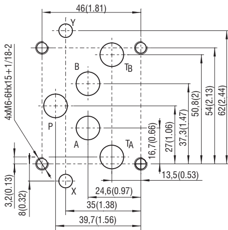
Ports P, A, B, T - max Ø 11.2 mm (0.44 in)
